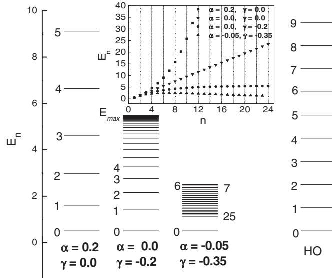
Figure 1. Energy levels for Hamiltonian (32) for several values of the parameters \alpha and \gamma . One sees dilation and compression of the spectrum, compared to the harmonic oscillator, on the right. In the inserted figure one has the energies on the same scale.
